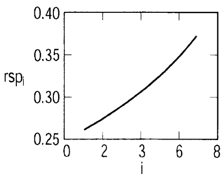
element reflection as funct. of tap #
