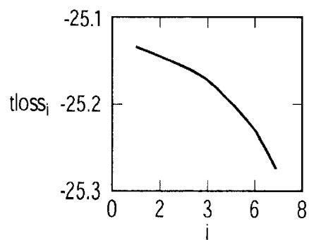
Transm. loss as funct. of tap #, dB
