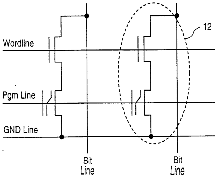
FIG. 2 (PRIOR ART)
