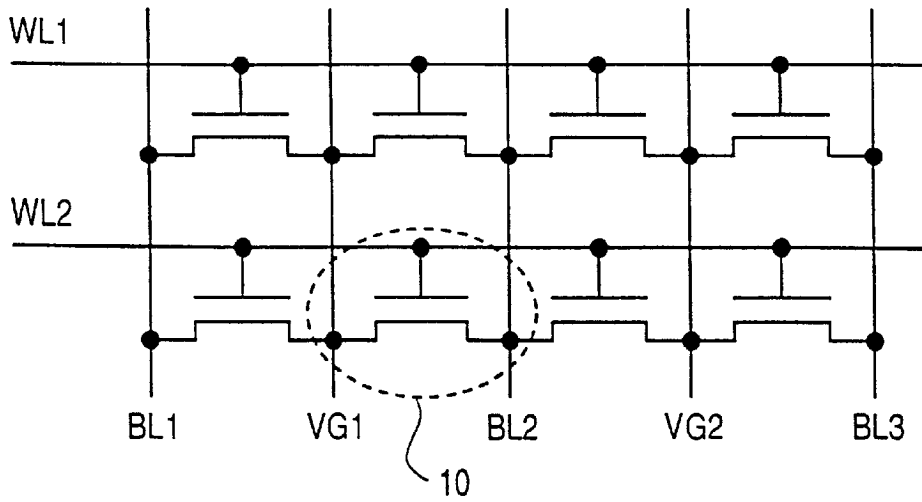
FIG. 1 (PRIOR ART)
